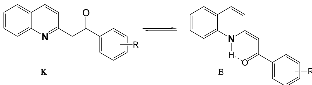
Scheme 3. tautomeric equilibria in 2- ketomethylquinoline
