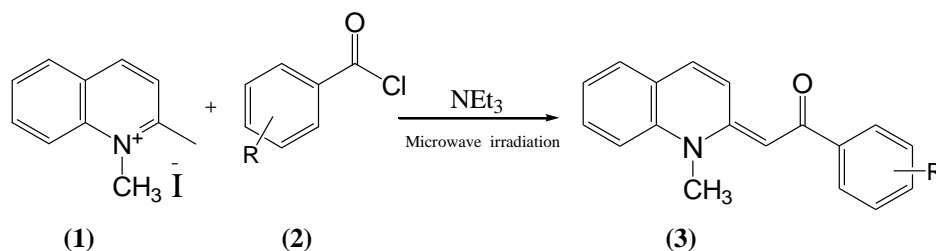
Scheme 2. Preparation of N-alkyl 2-ketomethylquinoline under microwave irradiation
