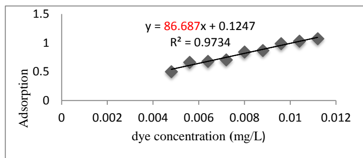
Fig 2. Calibration Curve of Erythrosine
