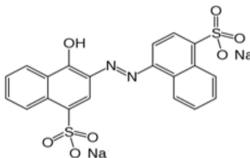
Scheme 2. The molecular structure of Red Carmoisine
